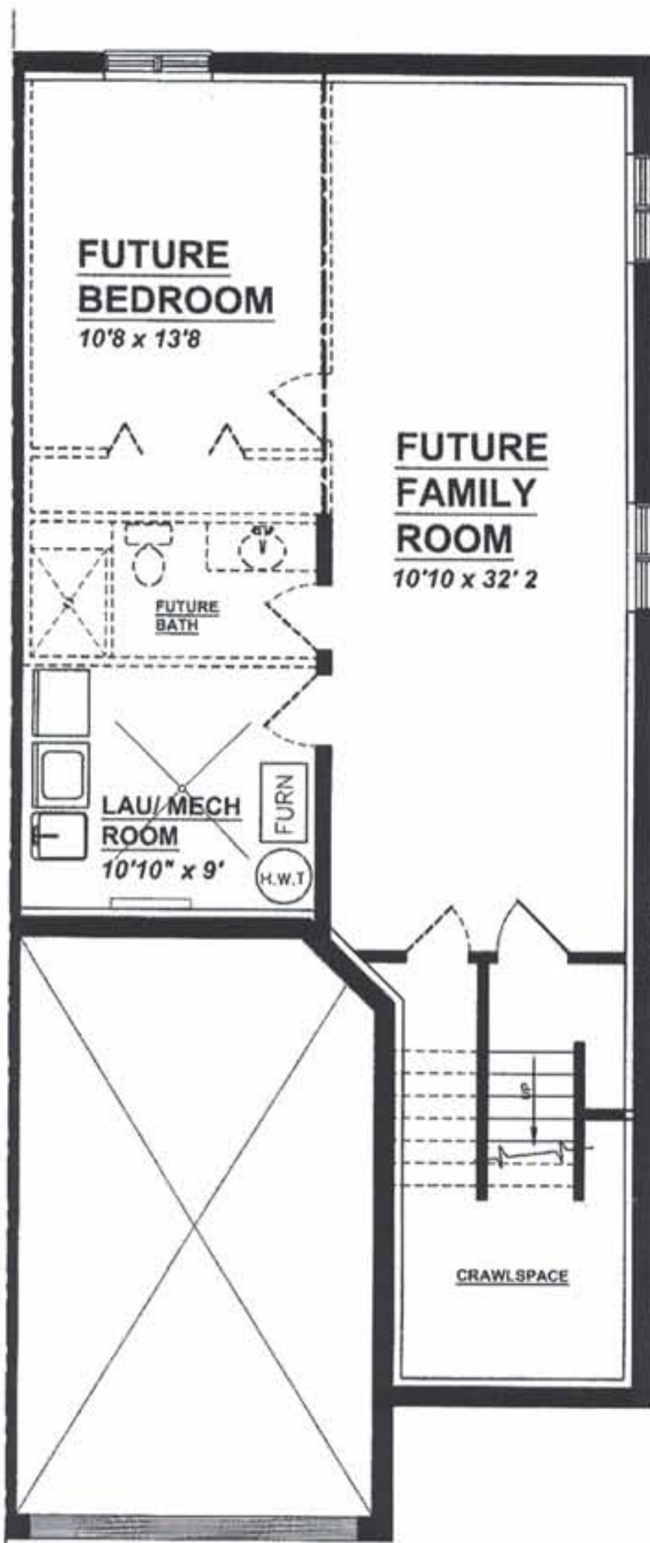
FOUNDATION PLAN
